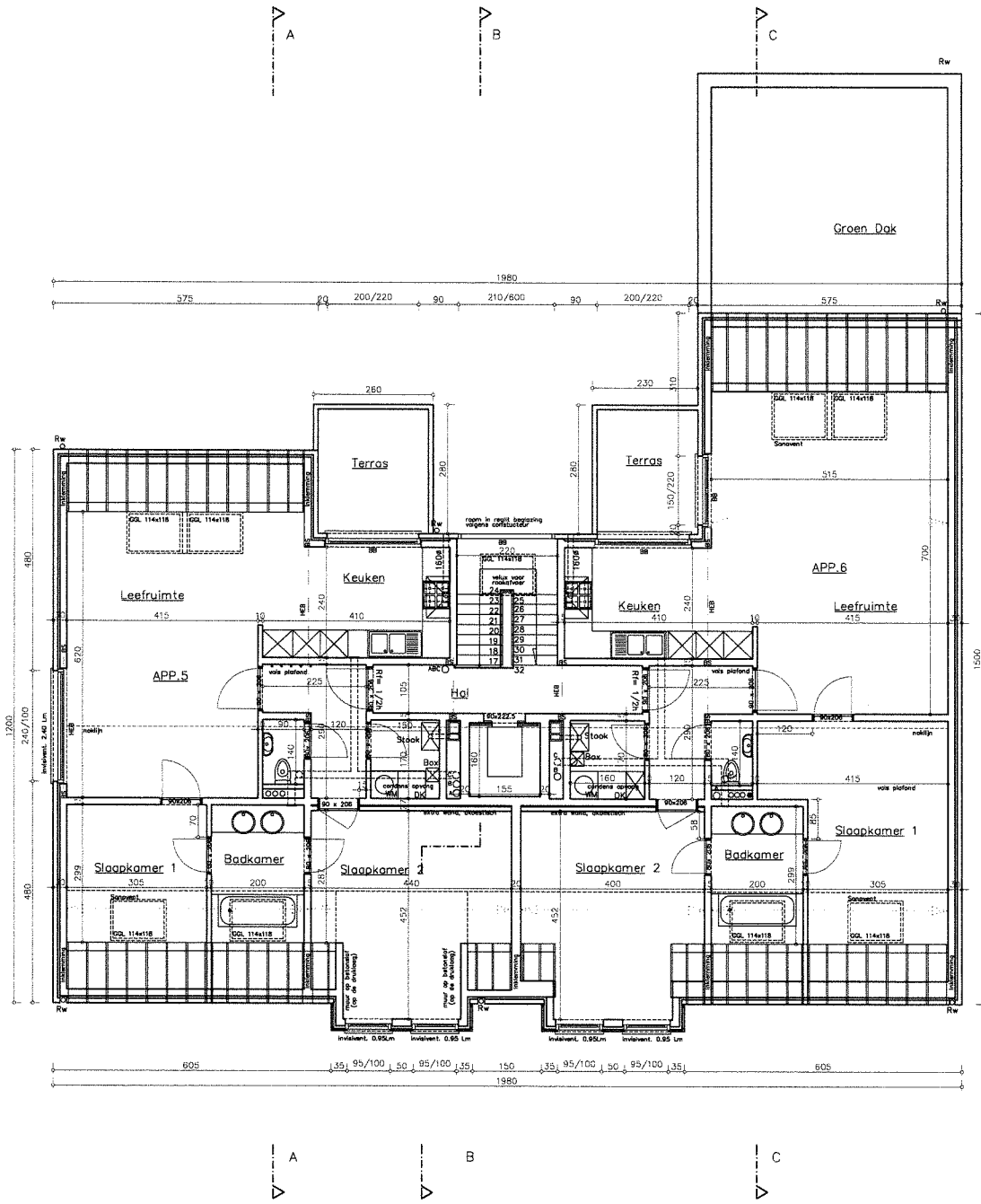
PLAN DAKVERDIEPING
